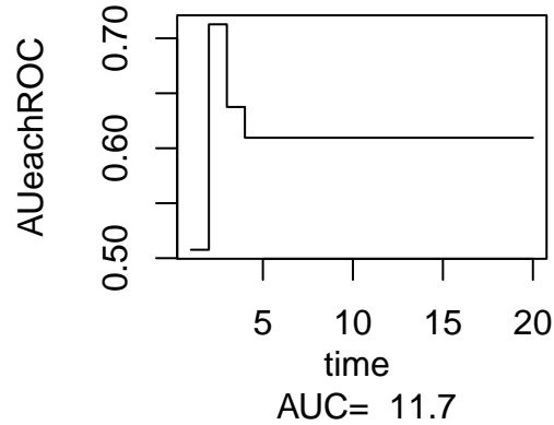
Figure 6: AURC curve
